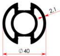
MK21D 1,145 kg/m
