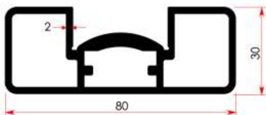
MK30 1.661 kg/m
